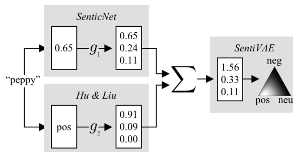
Figure 1: A depiction of the “encoder” portion of SentiVAE. The word peppy has polarity values of 0.65 and pos in the SenticNet and Hu-Liu lexica, respectively. These values are “encoded” into two three-dimensional vectors, which are then summed and added to (1, 1, 1) (not shown) to form the parameters of a Dirichlet over the latent representation of the word’s polarity value.
